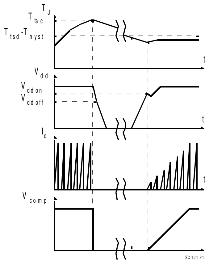
Figure 13. Over-temperature protection
