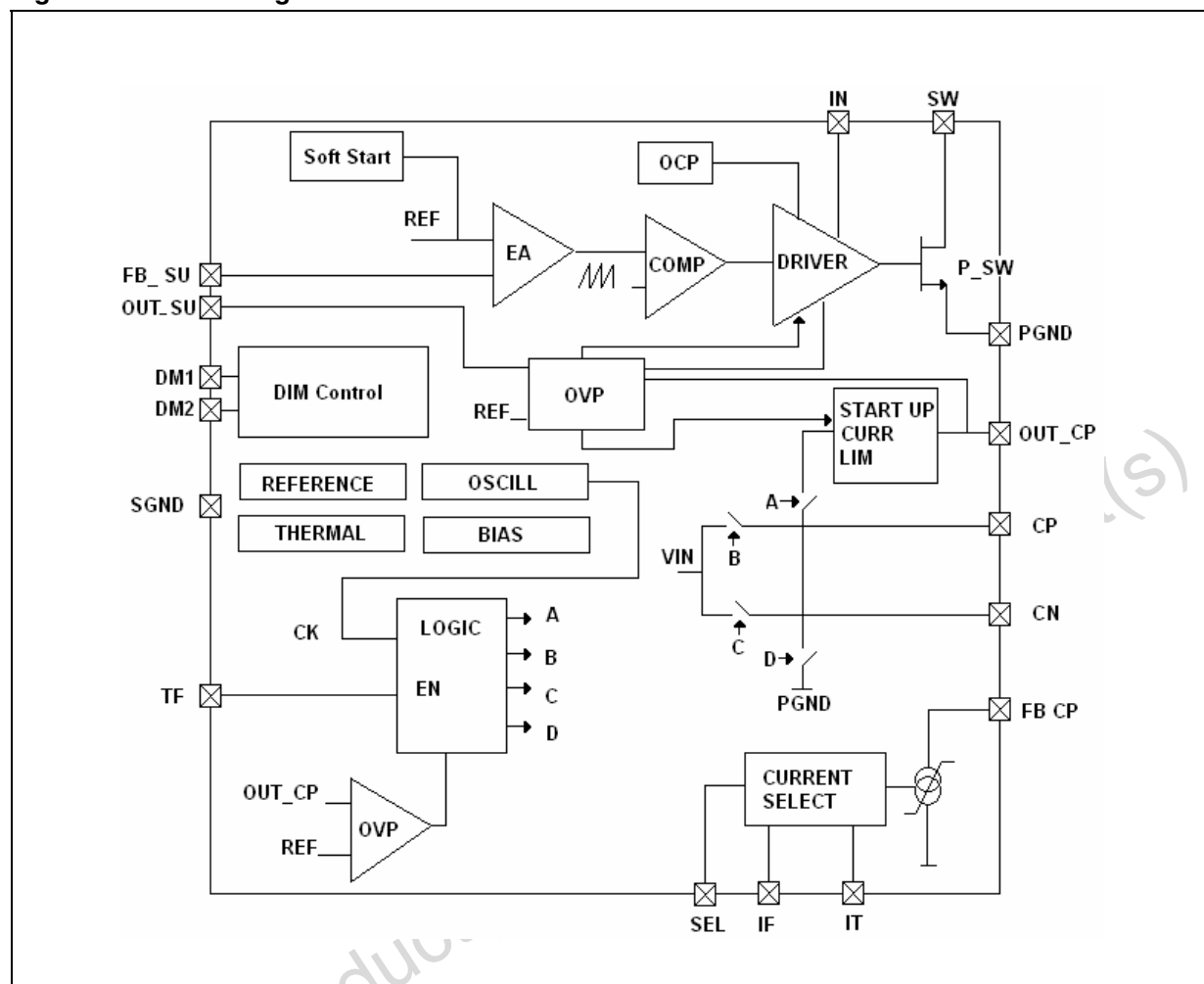
Figure 1. Block diagram
