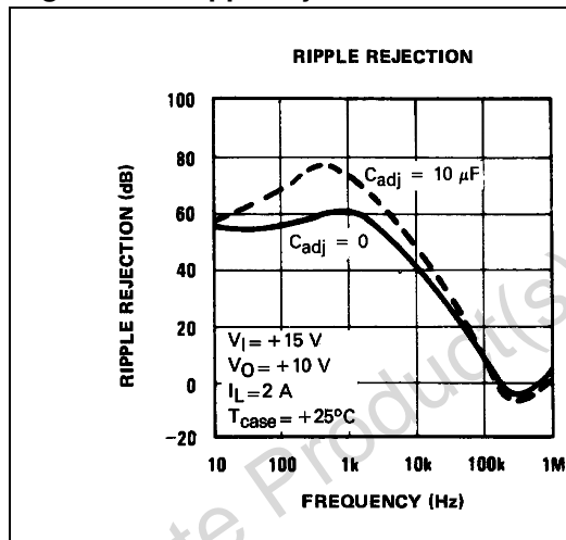
Figure 13. Ripple rejection
