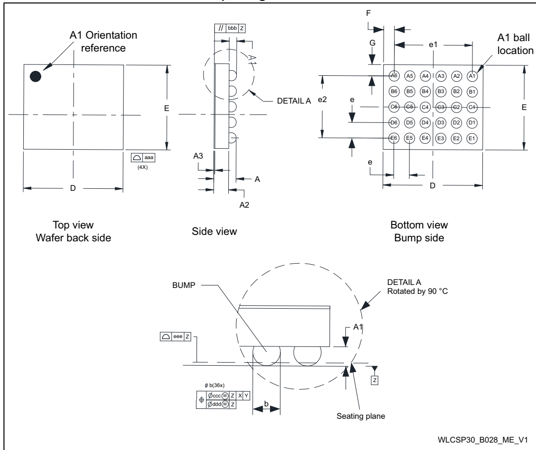
Figure 34. WLCSP30 30-ball, 3.065 x 2.865 mm, 0.5 mm pitch wafer level chip scale package outline
