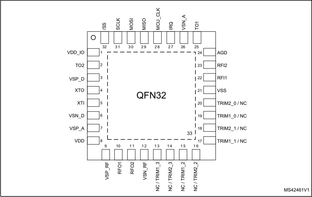
Figure 29. ST25R3912/3 QFN32 pinout (1)
