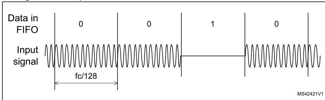
Figure 28. Example of Tx in Stream Mode for stx = 000b and OOK modulation
