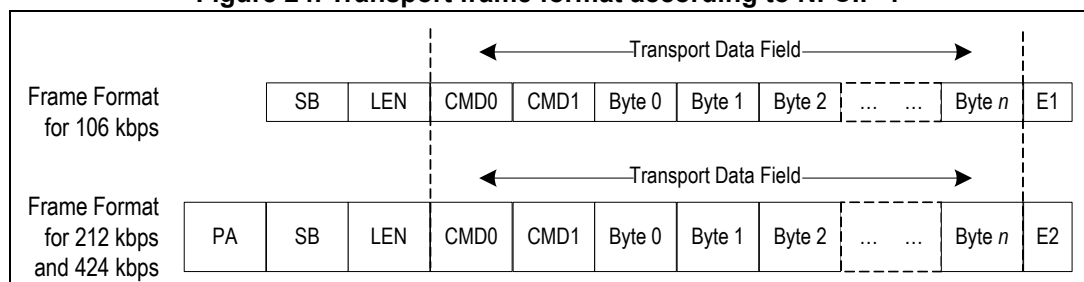
Figure 24. Transport frame format according to NFCIP-1
