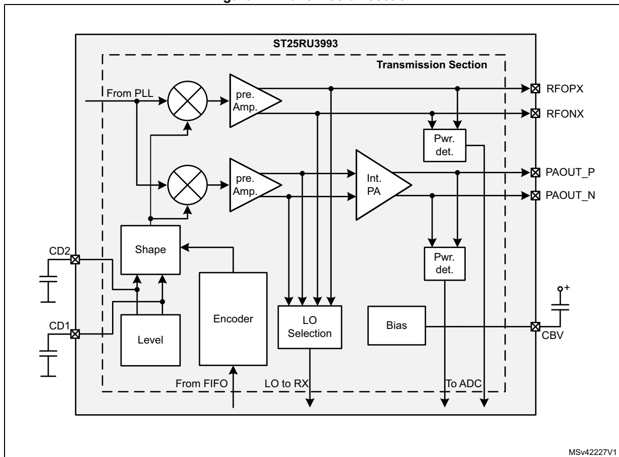
Figure 11. Transmission section
