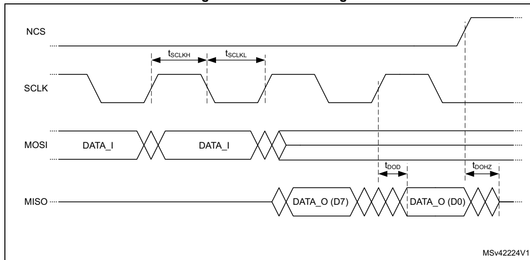
Figure 9. SPI Read timing
