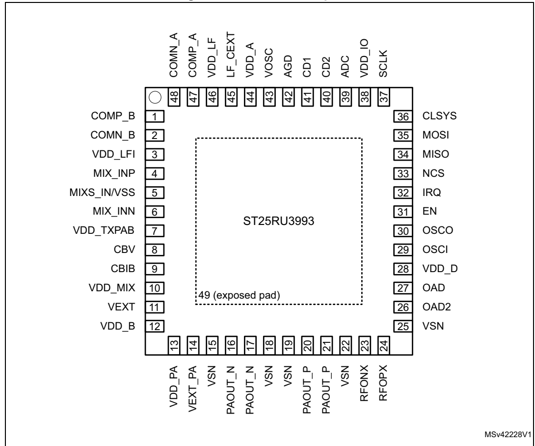
Figure 13. ST25RU3993 pinout
