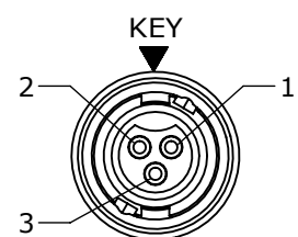
FACE VIEW P/N: CA162803PXXX90
