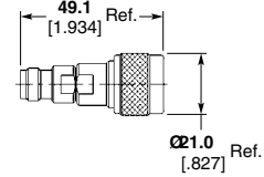
TNC Jack – N Series Plug
