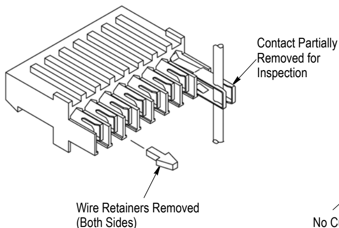
Terminated Test Connector
