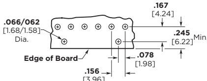
Recommended Mounting Hole Pattern for .062 [1.57] Thick PC Board Using a Straight Post Header
