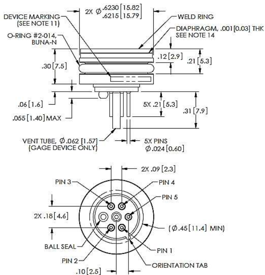
Sensor Pinout
