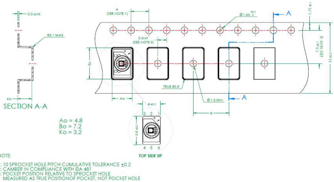
Figure 20: Tape & reel
