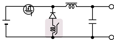
Chopper Converter
