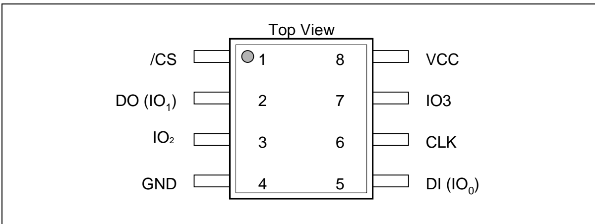
Figure 1a. W25Q64JV Pin Assignments, 8-pin SOIC 208-mil (Package Code SS)
