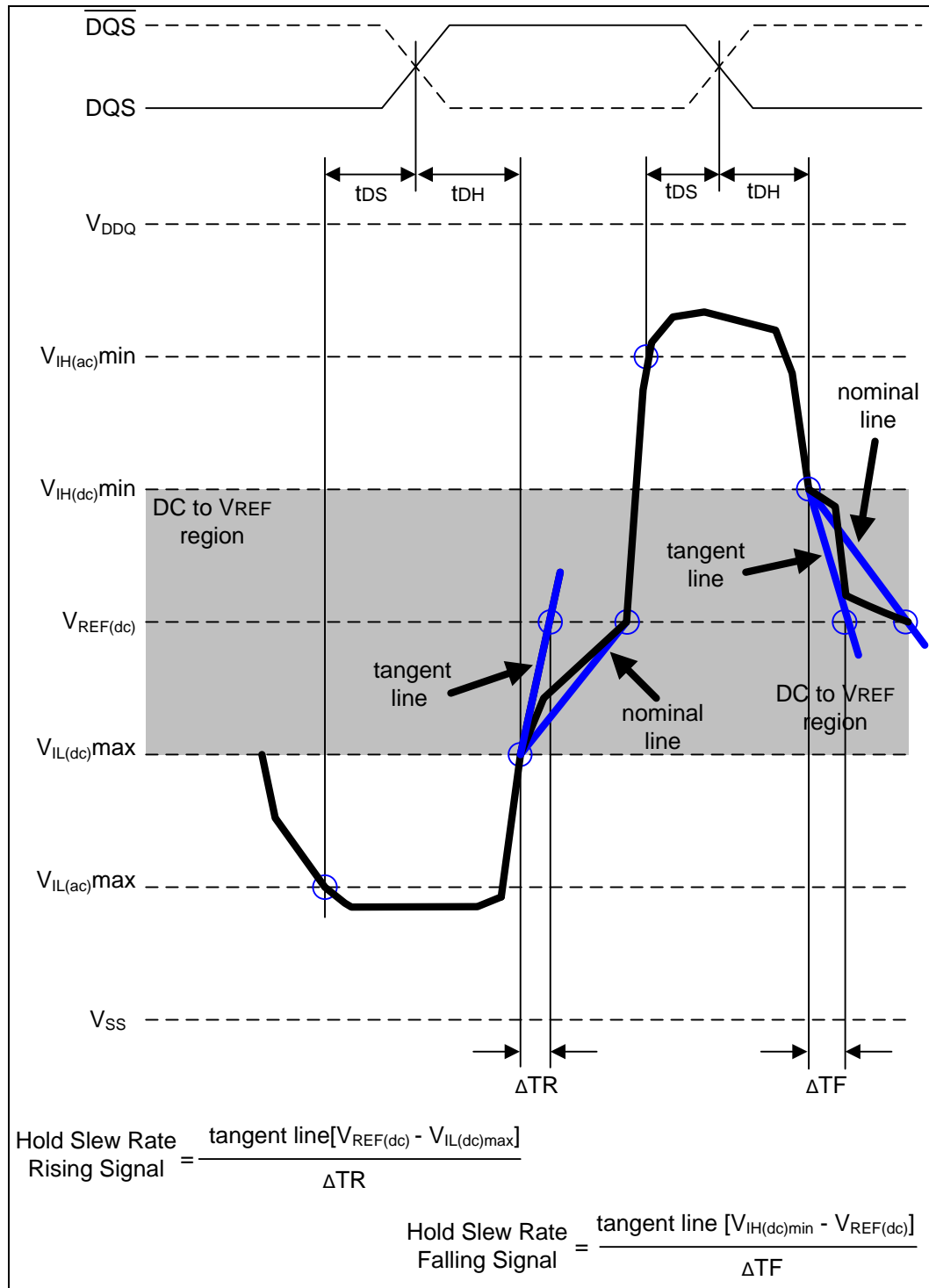
Figure 27 – Illustration tangent line for t_{DH} (differential \text{DQS}, \overline{\text{DQS}} )
