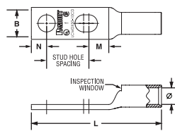
Figure 2. Two-Hole Slotted
