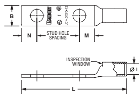
Figure 1. Two-Hole
