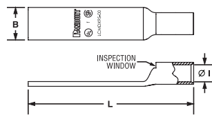
Figure 3. Blank Tongue
