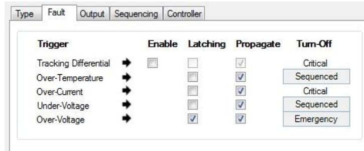
Figure 31. GUI dPOL Fault Latching and Propagation Option Window
