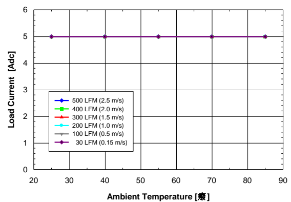
Figure 2. Available output current vs. ambient air temperature and airflow rates for converter DP8105G mounted horizontally with air flowing from input to output, MOSFET temperature \leq 120 °C, V_{in} = 12 V, V_{out} = 5 V, and F_{sw} = 1 MHz
