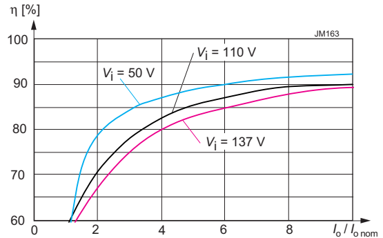
Fig. 10b Efficiency versus input voltage and load. Typical values (110IMY70-05)
