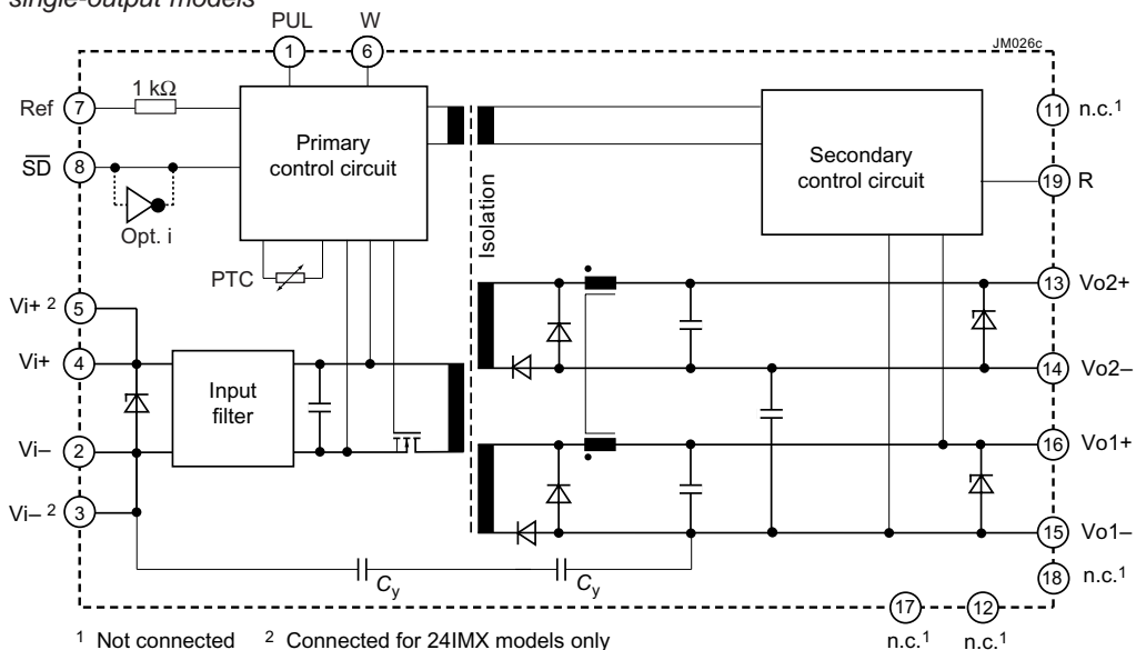
Block diagram of double-output models
