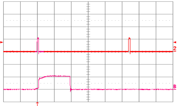
Figure 25. Load current (top trace, 20 A/div, 20 ms/div) into a 10 mΩ short circuit during restart, at V_{in} = 24 V. Bottom trace (20 A/div, 1 ms/div) is an expansion of the on-time portion of the top trace.
