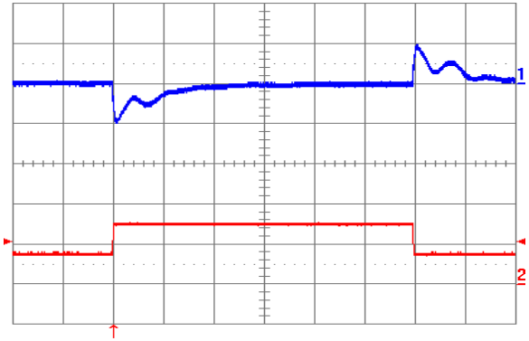
Figure 19. Output voltage response to load current step-change (3.75 A – 7.5 A – 3.75 A) at V_{in} = 24 V. Top trace: output voltage (100 mV/div). Bottom trace: load current (5 A/div). Current slew rate: 5 A/ \mu s. C_o = 450 \mu F tantalum + 1 \mu F ceramic. Time scale: 0.2 ms
