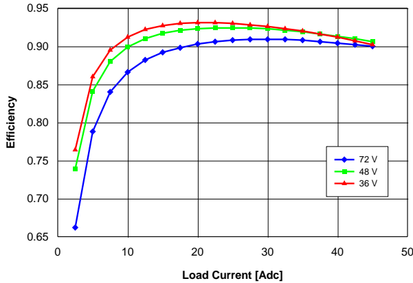
Fig. 3.3V.3: Efficiency vs. load current and input voltage for converter mounted vertically with air flowing from pin 3 to pin 1 at a rate of 300 LFM (1.5 m/s) and T_a = 25\text{ }^\circ\text{C} .
