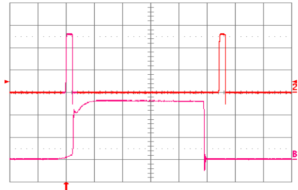
Fig. 1.2V.15: Load current (top trace, 20 A/div, 20 ms/div) into a 10 mΩ short circuit during restart, at Vin = 48 V. Bottom trace (20 A/div, 1 ms/div) is an expansion of the on-time portion of the top trace.
