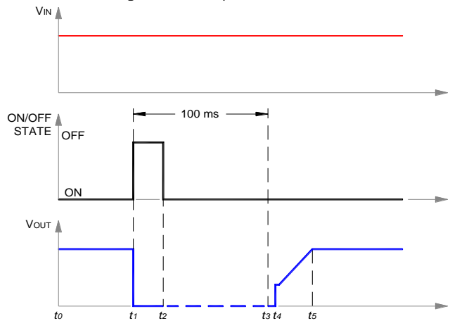
Figure 8. Startup scenario #3.
