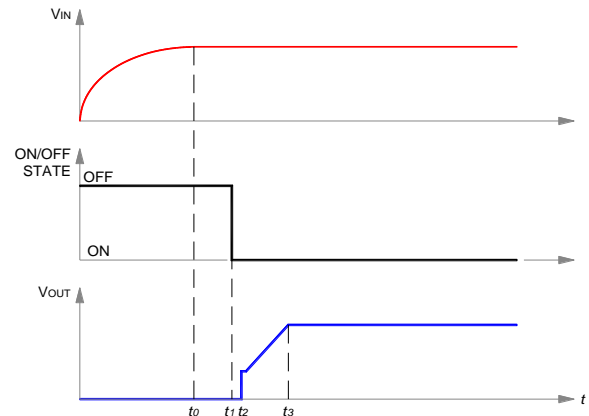
Figure 7. Startup scenario #2.
