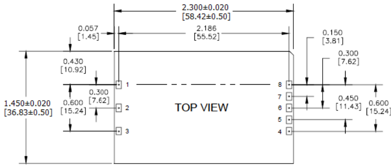
QMS48 (SurfaceMount)
