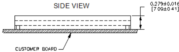
QMS48 (SurfaceMount)
