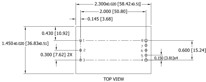
QM48T (Through-Hole)
