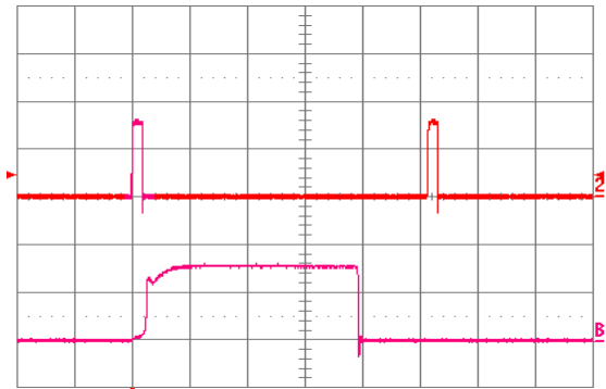
Figure 25. Load current (top trace, 20 A/div, 20 ms/div) into a 10 m\Omega short circuit during restart, at V_{in} = 48 V. Bottom trace (20 A/div, 1 ms/div) is an expansion of the on-time portion of the top trace.
