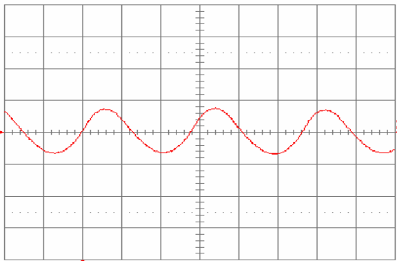
Fig. 13: Input reflected ripple current, i_c (500 mA/div.), measured at input terminals at full rated load current and V_{in} = 48 \text{ V} . Refer to Fig. 12 for test setup. Time scale: 1 \mu\text{s}/\text{div} .
