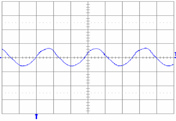
Fig. 11: Output voltage ripple (50 mV/div.) at full rated load current into a resistive load with C_o = 10 \mu\text{F} tantalum + 1 \mu\text{F} ceramic and V_{in} = 48 \text{ V} . Time scale: 1 \mu\text{s}/\text{div} .
