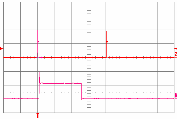
Fig. 16: Load current (top trace, 20 \text{ A}/\text{div} ., 50 \text{ ms}/\text{div} .) into a 10 \text{ m}\Omega short circuit during restart, at V_{in} = 48 \text{ V} . Bottom trace ( 20 \text{ A}/\text{div} ., 2 \text{ ms}/\text{div} .) is an expansion of the on-time portion of the top trace.
