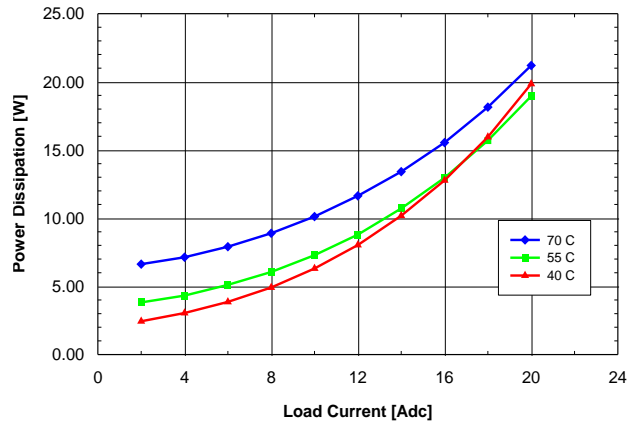
Fig. 6: Power dissipation vs. load current and ambient temp. for converter mounted vertically with V_{in} = 48\text{ V} and air flowing from pin 1 to pin 3 at a rate of 200 LFM (1.0 m/s).
