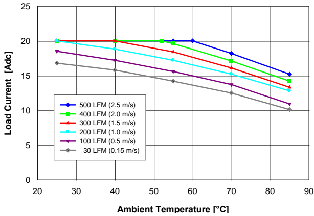
Fig. 1 : Available load current vs. ambient air temperature and airflow rates for converter with G height pins mounted vertically with air flowing from pin 1 to pin 3, MOSFET temperature \leq 125 °C, V_{in} = 48 V.
