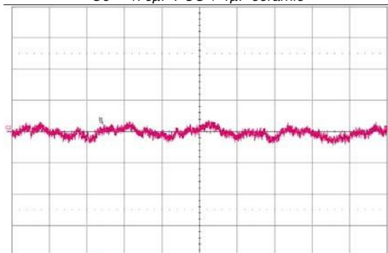
Figure 14. Input reflected-ripple current, i_{\text{is}} (10 mA/div.), measured through 10 \mu\text{H} at the source at full rated load current and V_{\text{in}} = 48\text{V} . Refer to Fig. J for test setup. Time scale: 1 \mu\text{s} /div.
