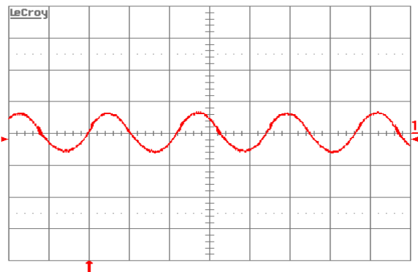
Figure 13: Input reflected-ripple-current, i_c (200 mA/div.), through 10 \mu\text{H} measured at input terminals at full rated load current and V_{in} = 48 \text{ V} . Refer to Figure 11 for test setup. Time scale: 1 \mu\text{s}/\text{div} .
