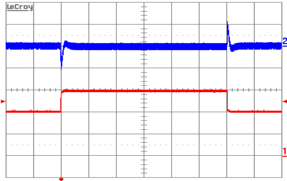
Figure 9: Output voltage response to load current step-change (10A–15A–10A) at V_{in}=48\text{V} . Top trace: output voltage (100 mV/div.). Bottom trace: load current (5A/div.). Current slew rate: 5\text{A}/\mu\text{s} . C_o= 470\mu\text{F} POS + 1\mu\text{F} ceramic. Time scale: 0.2 mS/div.
