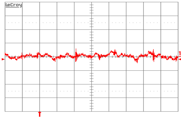
Figure 12: Input reflected-ripple current, i_s (10 mA/div.), measured 10 \mu\text{H} at the source at full rated load current and V_{in} = 48 \text{ V} . Refer to Figure 11 or test setup. Time scale: 1 \mu\text{s}/\text{div} .
