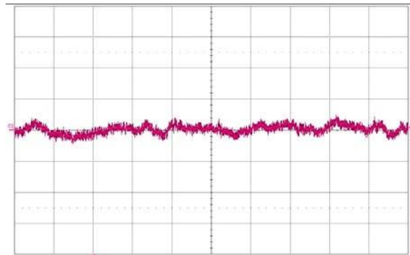
Figure 14. Input reflected-ripple current, i_s (10 mA/div.), measured through 10 \mu\text{H} at the source at full rated load current and V_{in} = 48 V. Refer to Fig. J for test setup. Time scale: 1 \mu\text{s}/\text{div} .
