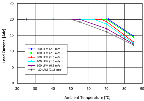
Figure 1. Available load current vs. ambient air temperature and airflow rates for SSQL48T20033 converter mounted vertically with air flowing from pin 3 to pin 1, TC temperatures \leq 120^\circ\text{C} , V_{in} = 48\text{ V} .
