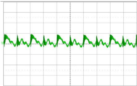
Figure 13. Output voltage ripple (20 mV/div.) at full rated load current into a resistive load with C_o = 10 \mu\text{F} tantalum + 1 \mu\text{F} ceramic and V_{in} = 48 V. Time scale: 2 \mu\text{s}/\text{div} .
