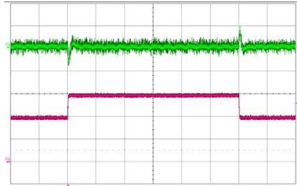
Figure 12. Output voltage response to load current step change (10 A – 15 A – 10 A) at V_{in} = 48 V. Top trace: output voltage (100 mV/div.) Bottom: load current (5 A/div.). Current slew rate: 1 \text{ A}/\mu\text{s} . Time scale: 200 \mu\text{s}/\text{div} . C_o = 470 \mu\text{F} POS + 1 \mu\text{F} ceramic
