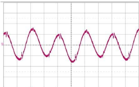
Figure 15. Input reflected ripple-current, i_c (50 mA/div.), measured at input terminals at full rated load current and V_{in} = 48 V. Refer to Fig. J for test setup. Time scale: 1 \mu\text{s}/\text{div} .
