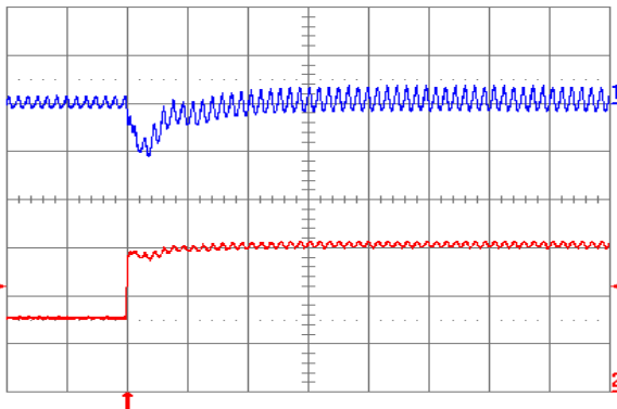
Fig. 1.2V.7: Output voltage response for V_{out} = 1.2\text{ V} to positive load current step change from 2.5 A to 5 A with slew rate of 5 A/ \mu\text{s} at V_{in} = 5\text{ V} . Top trace: output voltage (100 mV/div.); Bottom trace: load current (2 A/div.). C_o = 47\text{ }\mu\text{F} ceramic + 1 \mu\text{F} ceramic. Time scale: 20 \mu\text{s} /div.
