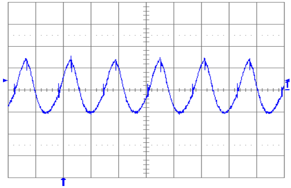
Fig. 1.2V.6: Output voltage ripple (20 mV/div.) at full rated load current into a resistive load with external capacitance 10 \mu\text{F} ceramic + 1 \mu\text{F} ceramic and V_{in} = 5\text{ V} for V_{out} = 1.2\text{ V} . Time scale: 2 \mu\text{s} /div.
