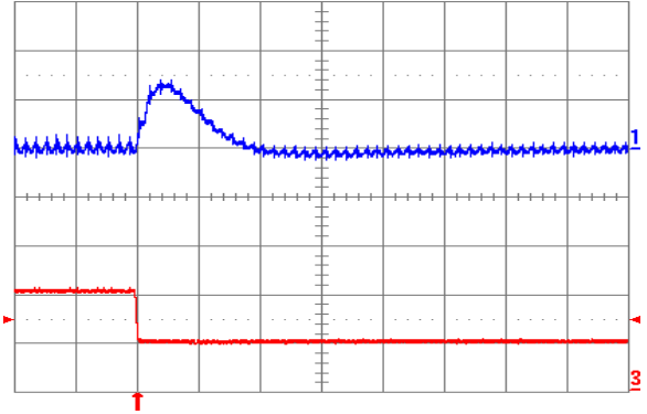
Fig. 2.0V.8: Output voltage response (YNL12S10020) to negative load current step change from 10 A to 5 A with slew rate of -5 A/μs at V_{in} = 12\text{ V} . Top trace: output voltage (100 mV/div.); Bottom trace: load current (5 A/div.). C_o = 100\text{ }\mu\text{F} ceramic. Time scale: 20 μs/div.
