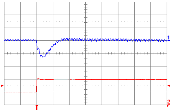
Fig. 1.5V.7: Output voltage response for V_{out} = 1.5\text{ V} to positive load current step change from 5 A to 10 A with slew rate of 5\text{ A}/\mu\text{s} at V_{in} = 5\text{ V} . Top trace: output voltage (100 mV/div.); Bottom trace: load current (5 A/div.). C_o = 47\ \mu\text{F} ceramic + 1\ \mu\text{F} ceramic. Time scale: 20 \mu\text{s} /div.
