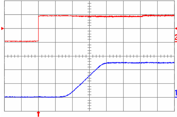
Fig. 2.5V.5: Turn-on transient for V_{out} = 2.5\text{ V} with the application of Enable signal at full rated load current (resistive) and 47\ \mu\text{F} external capacitance at V_{in} = 5\text{ V} . Top trace: Enable signal (2 V/div.); Bottom trace: output voltage (1 V/div.); Time scale: 2 ms/div.
