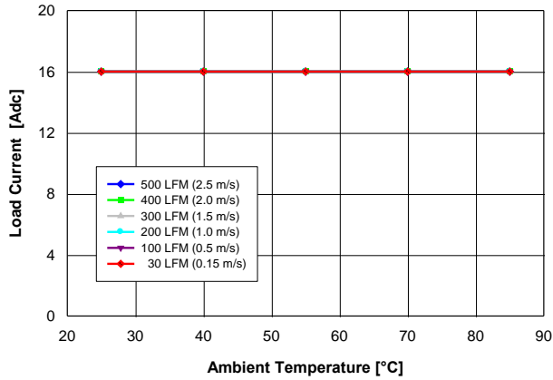
Fig. 0.7525V.1: Available load current vs. ambient temperature and airflow rates for V_{out} = 0.7525\text{ V} converter mounted vertically with V_{in} = 5\text{ V} , and maximum MOSFET temperature \leq 120\text{ }^{\circ}\text{C} .
