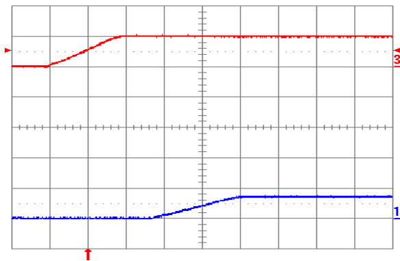
Fig. 0.7525V.5: Turn-on transient for V_{out} = 0.7525\text{ V} with application of V_{in} at full rated load current (resistive) and 100\text{ }\mu\text{F} external capacitance at V_{in} = 5\text{ V} . Top trace: V_{in} (5 V/div.); Bottom trace: output voltage (1 V/div.); Time scale: 2 ms/div.
