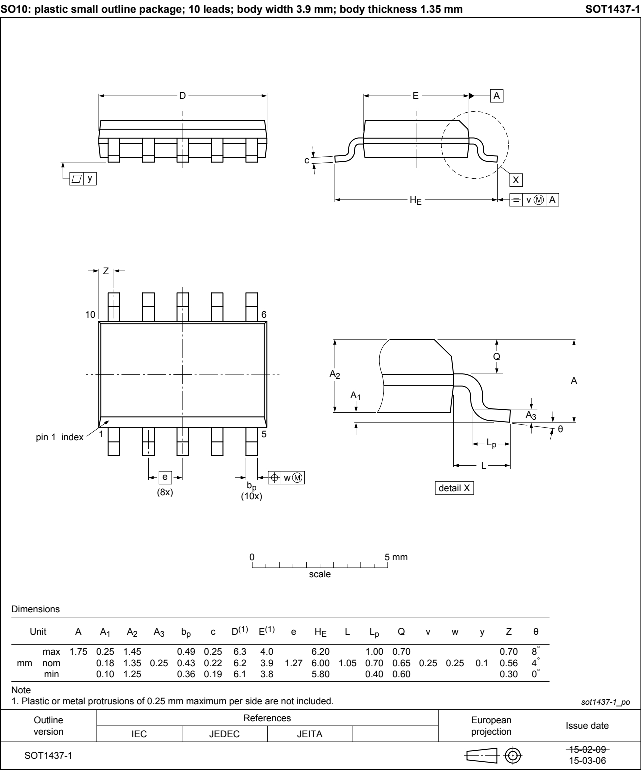
Figure 24. Package outline SOT1437-1 (SO10)
