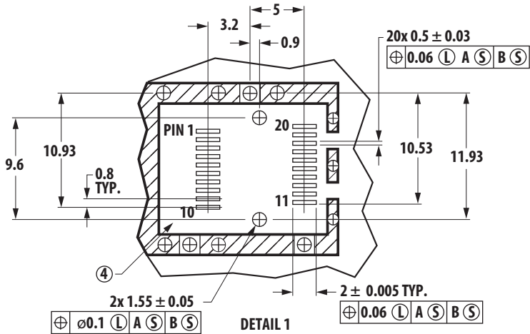
Figure 7. SFP Host Board Mechanical Layout
