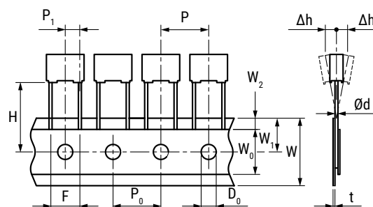
Figure 2 – Lead Spacing 7.5 mm
