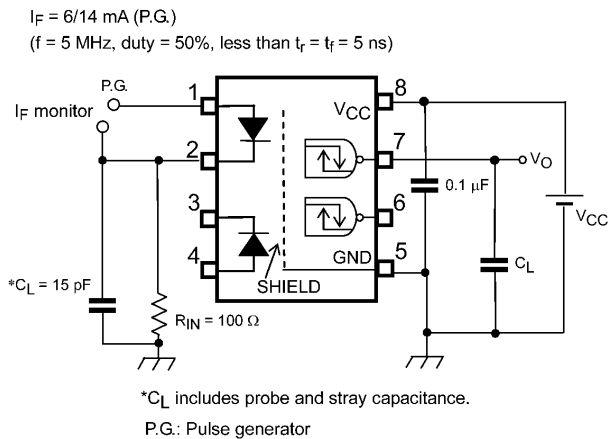
Fig. 12.1.5 Switching Time Test Circuit
