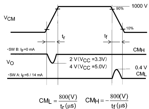
Fig. 12.1.6 Common-Mode Transient Immunity
