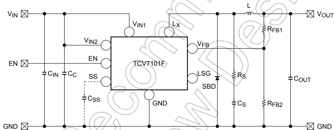
Figure 1 TCV7101F Typical Application Circuit Examples
