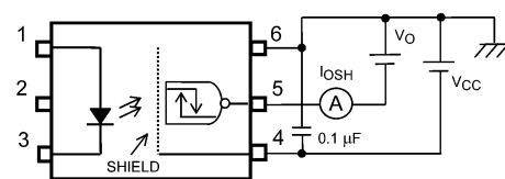
Fig. 12.1.6 IOSH Test Circuit
