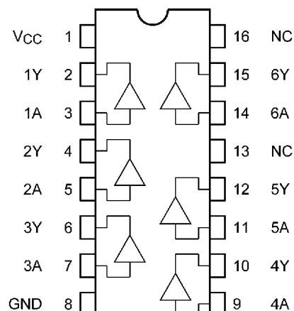
74HC4050D
