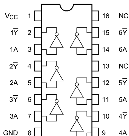
74HC4049D
