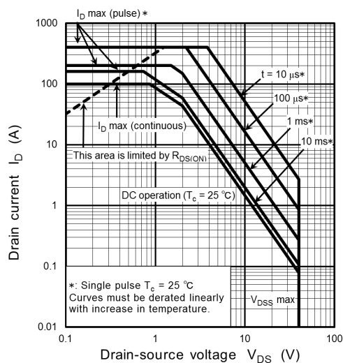
Fig. 8.15 Safe Operating Area (Guaranteed Maximum)
