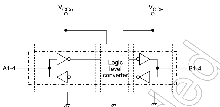
Fig. 6.1 Block Diagram
