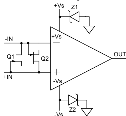
FIGURE 6. Overvoltage Protection
