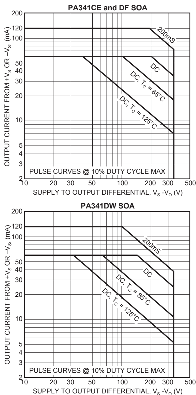
FIGURE 5. Safe Operating Area
