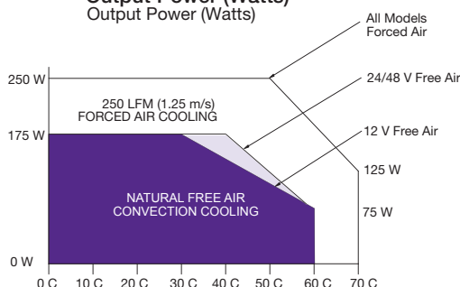
Figure 1b: Derating Curve With Cover Output Power (Watts) Output Power (Watts)
