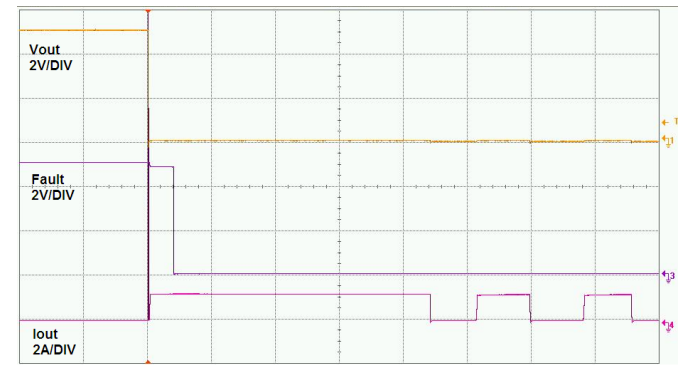
Figure 8 Extended Short-Circuit into Thermal Cycles
