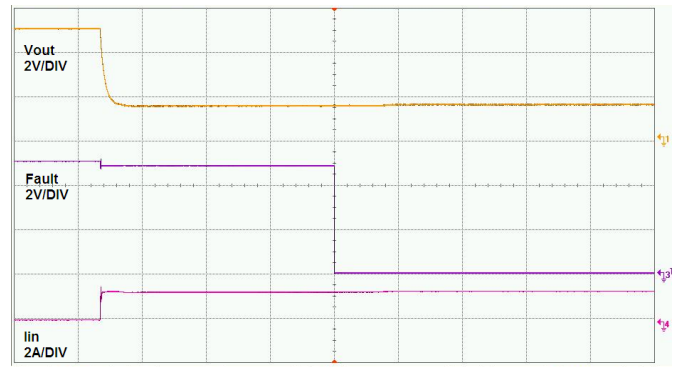
Figure 6 No Load to 1Ω Transient Response
