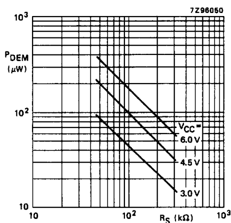
Fig.22 Typical dc power dissipation of demodulator section as a function of R_S ; R_1 = R_2 = \infty ; T_{\text{amb}} = 25 °C; V_{\text{VCOIN}} = 1/2 V_{\text{CC}} .
