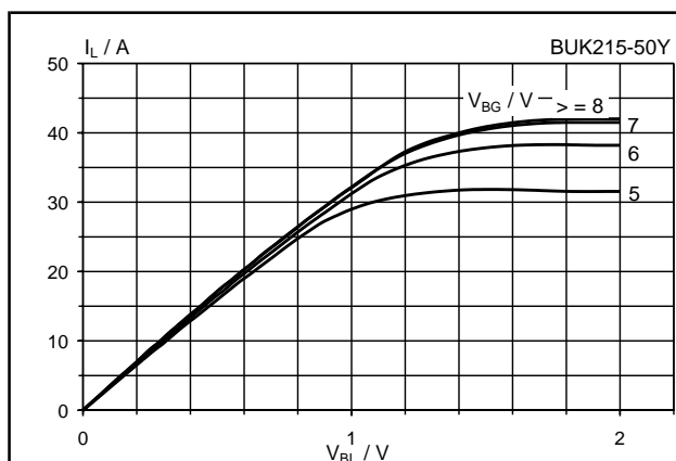
Fig.6. Typical on-state characteristics, T_j = 25 \text{ }^\circ\text{C} . I_L = f(T_j) ; parameter V_{BG} ; t_p = 250 \mu\text{s}
