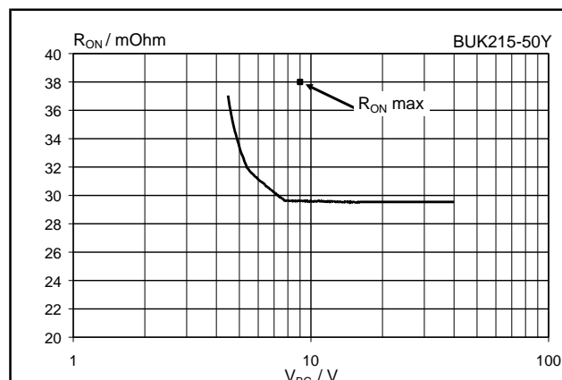
Fig.8. Typical on-state resistance, T_j = 25 \text{ }^\circ\text{C} . R_{ON} = f(V_{BG}) ; condition I_L = 10 \text{ A} ; t_p = 300 \mu\text{s}
