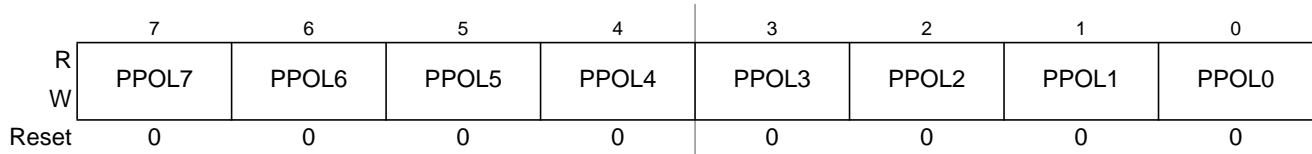
Figure 13-4. PWM Polarity Register (PWMPOL)
