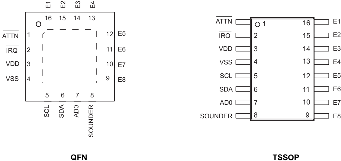
Figure 3. Package Pinouts
