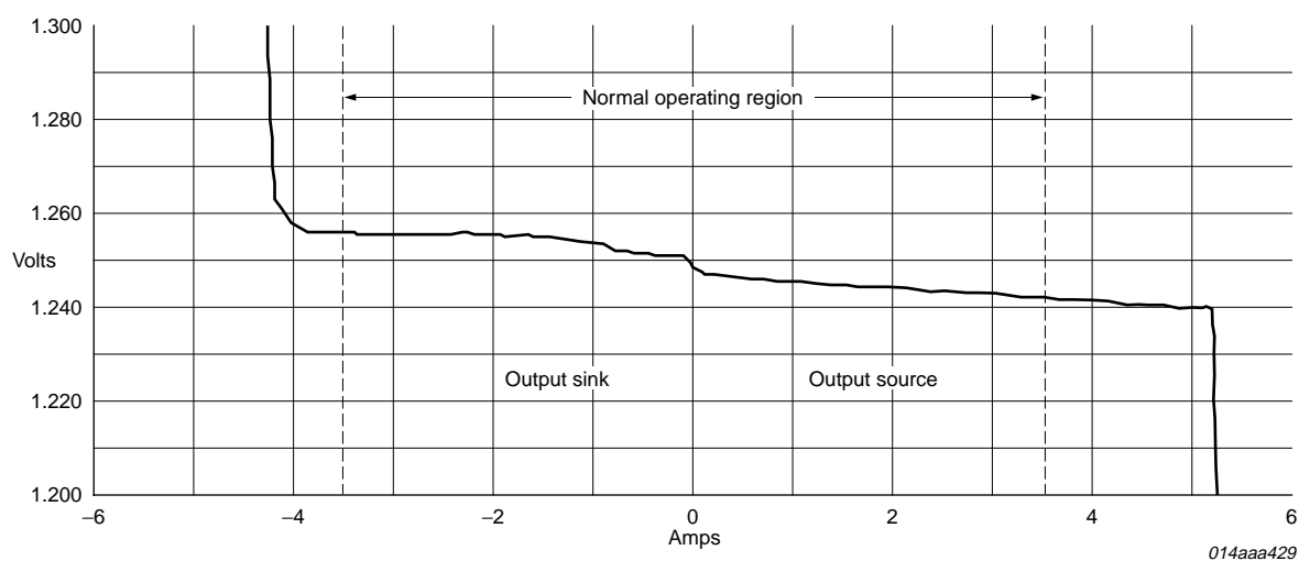
Fig 13. Typical V_{TT} versus output current ( V_{DD} = 2.5 V at 25^{\circ}\text{C} )
