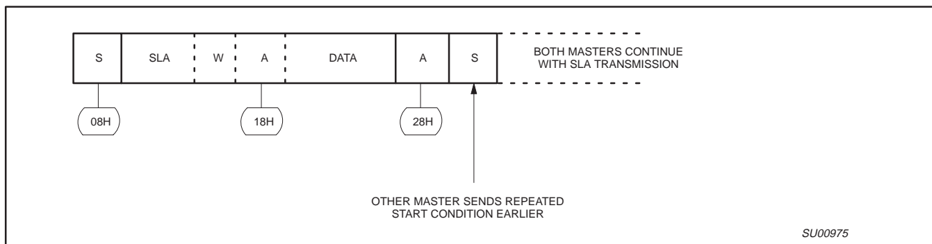
Figure 12. Simultaneous Repeated START Conditions from 2 Masters
