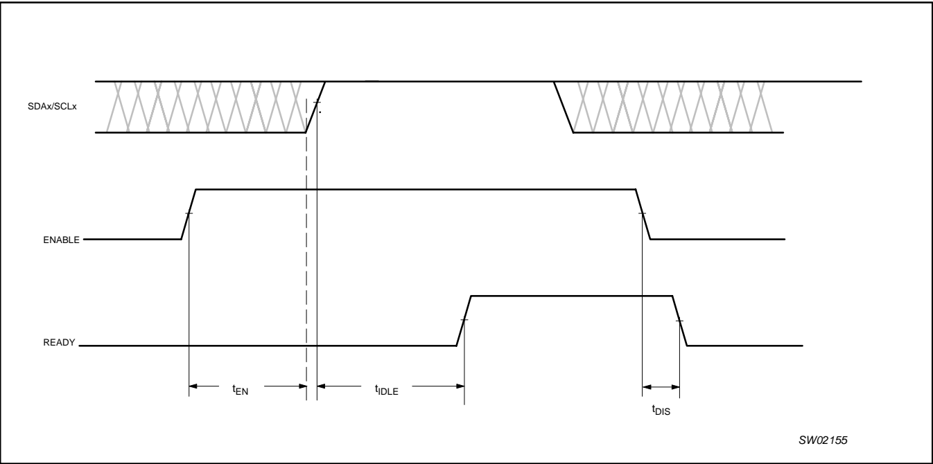
Figure 16. Timing for t_{ENABLE} , t_{IDLE} , and t_{DISABLE}
