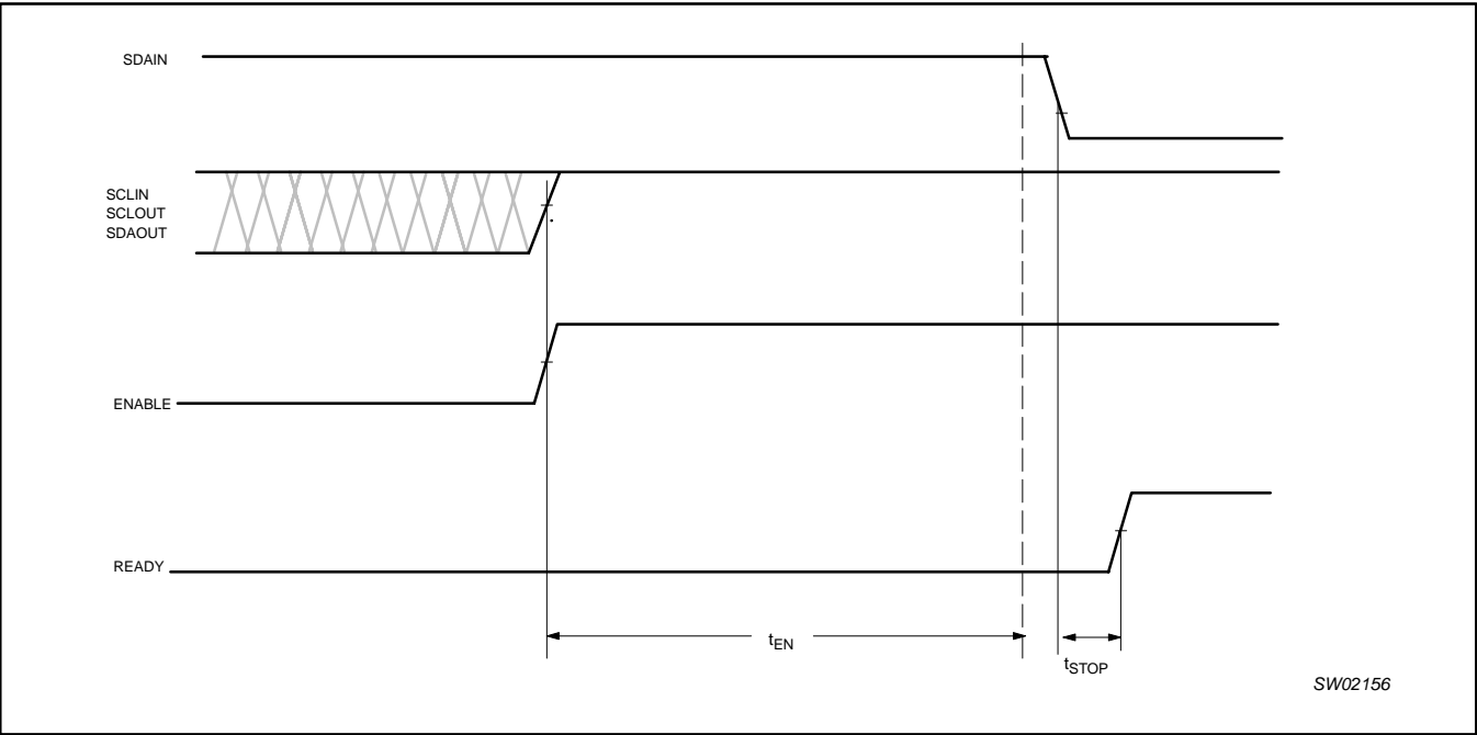
Figure 17. t_{STOP} that can occur after t_{ENALBE}
