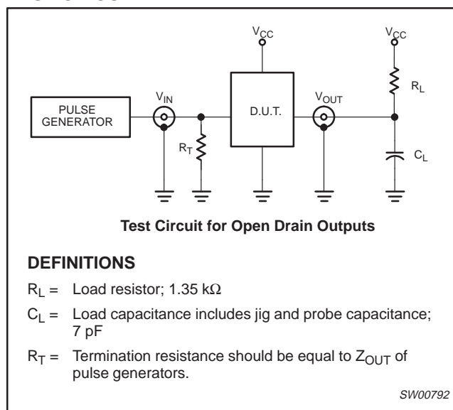
Figure 7. Test circuit
