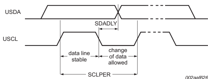
Fig 21. UFM I 2 C-bus bit transfer
