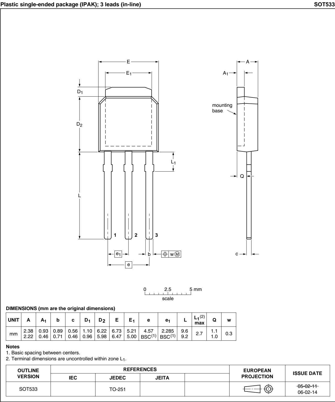
Fig 14. Package outline SOT533 (IPAK)
